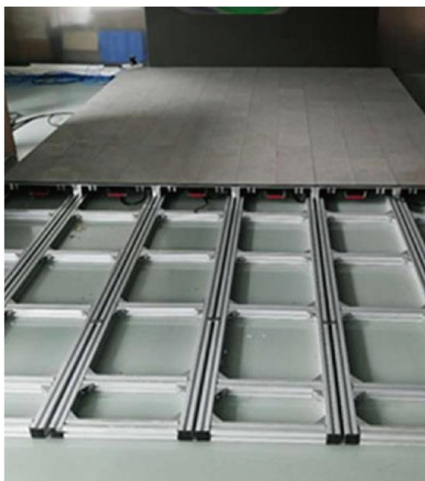
Guide rails
