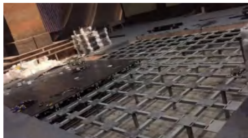
地托钢结构安装 Steel Structure Installation
