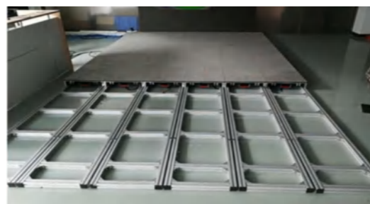
轨道安装 Guide rails installation
